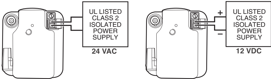
Figure 4. Power Supply Connections
